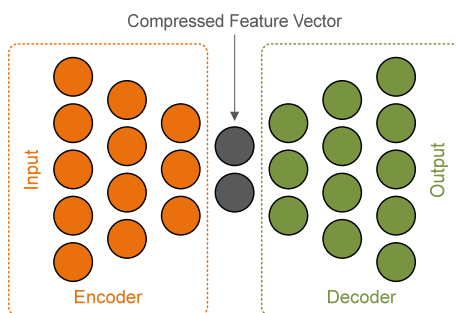
Figure 3 – ADM Autoencoder
