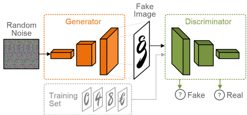
Figure 4 – GAN Architecture
