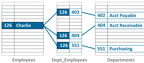
Figure 4 – Relational Data Model
