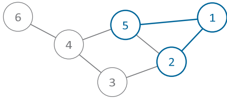
Figure 1 – Undirected Graph
