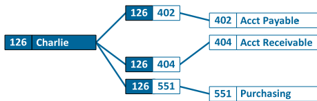
Figure 5 – Graph Data Model
